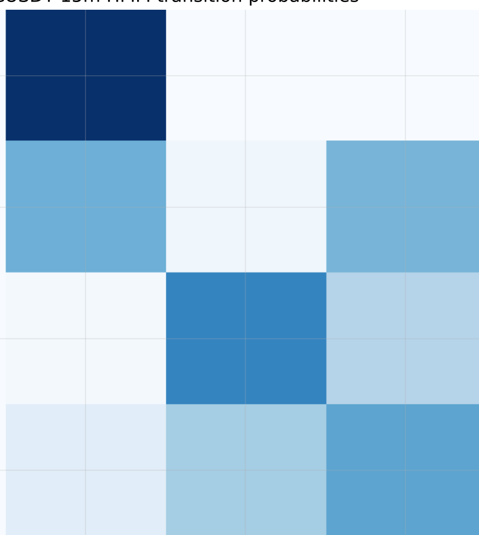
BTCUSDT 15m HMM transition probabilities
